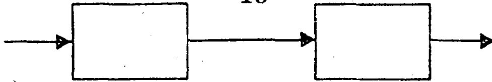
SEQUENCE
