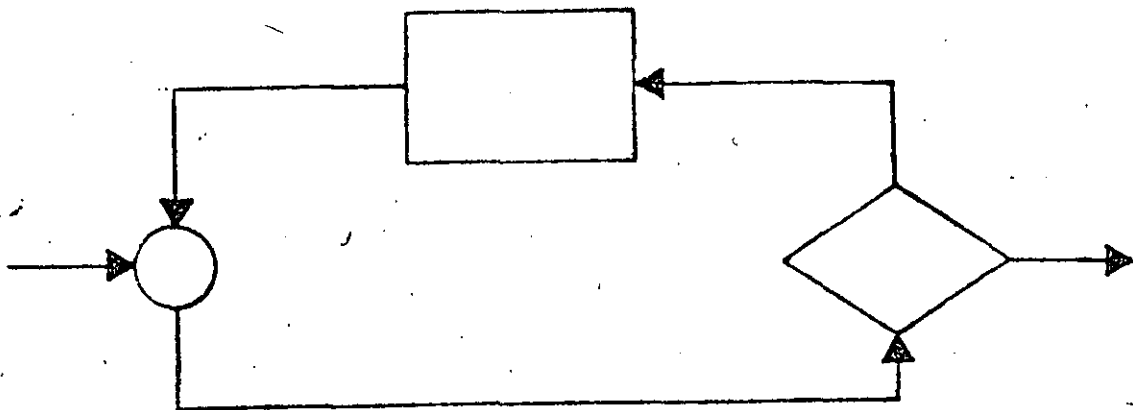
DOWHILE
