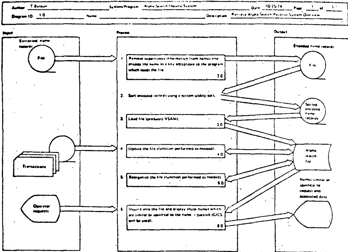
Figure 10. Alpha Search Inquiry System overview diagram (1.0)
