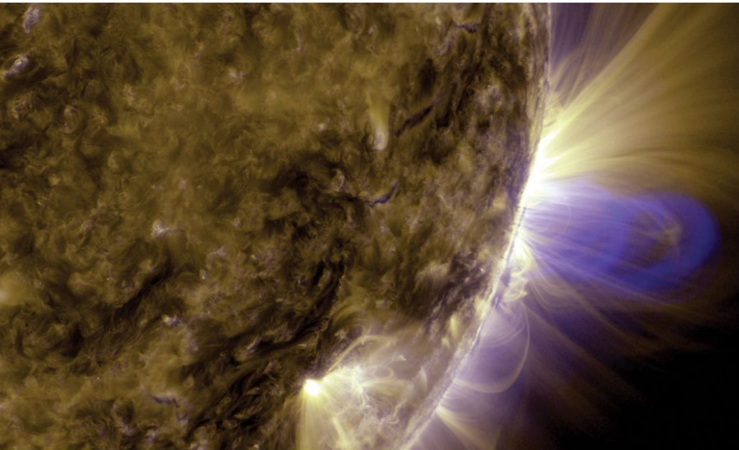
Above: Magnetic loops known as 'flux ropes' rise up from the Sun in this image from the Solar Dynamics Observatory.
