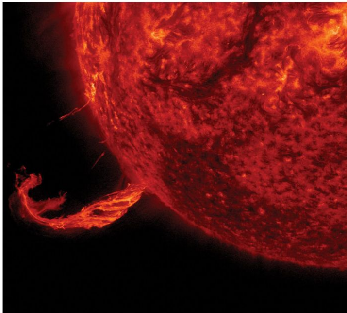
Above: This coronal mass ejection was recorded by the Solar Dynamics Observatory in February 2015. A substantial part shot off into space.
