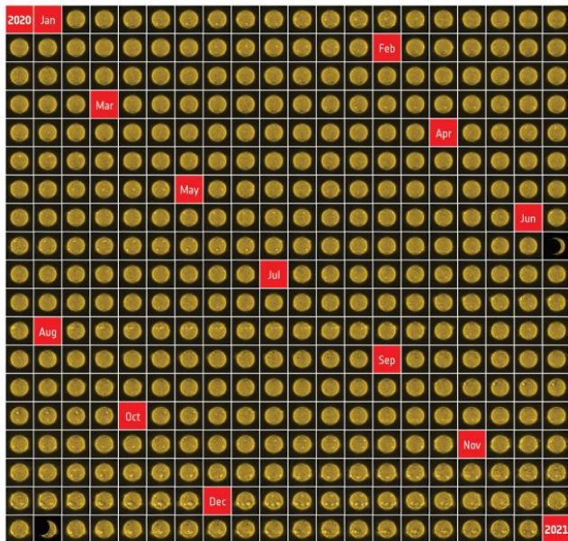
Above: These 366 images of the Sun, taken by the ESA's Proba-2 satellite, represent every day during 2020. Activity comes and goes, including two partial eclipses.
