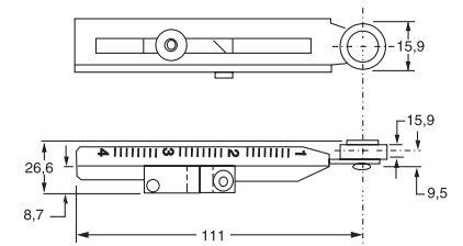
Brazo ajustable
