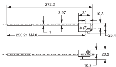
Varilla
