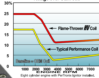
Percent of extra available voltage over OEM coil
