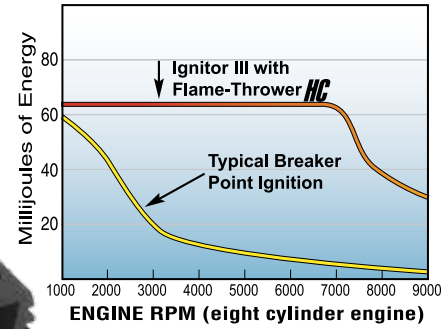
Ignitor III vs. Breaker Point Energy
