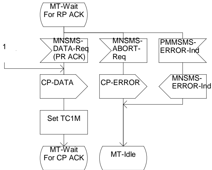
MT-SMC-GP entity on MS-side for GPRS SDL-17
