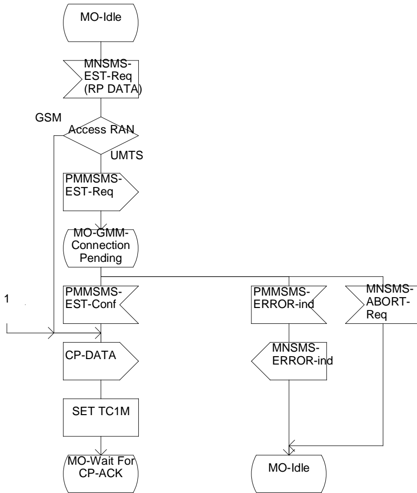
MO-SMC-GP entity on MS-side for GPRS SDL-13
