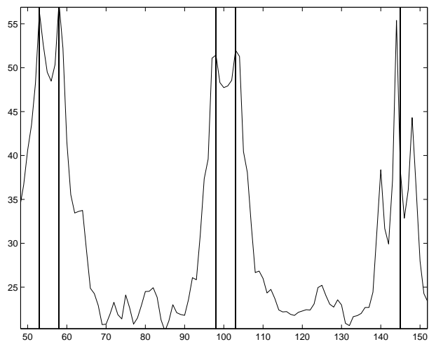
Fig. 8: The estimated spatial spectrum of the Multigroup sources using algorithm of [3] (Wider frequency band [300 : 3000])
