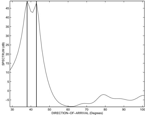
Fig. 3: The estimated spatial spectrum of the correlated sources using Modal Space Processing.
