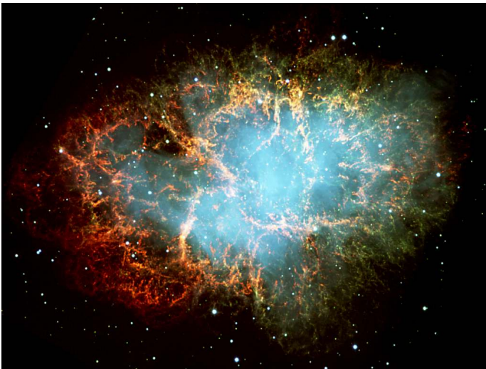
Figure 10: The Crab Nebula from VLT
