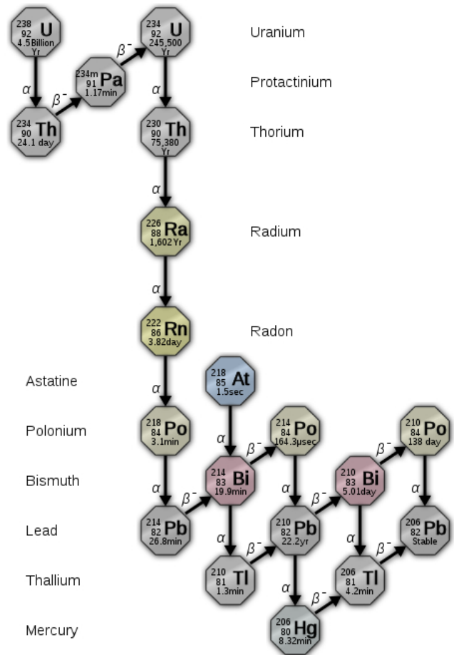
Figure 11: Uranium-238 decay series ending in Lead-206
