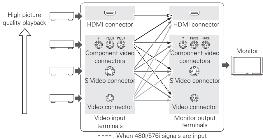
[Flow of video signals inside the AVR-989]
