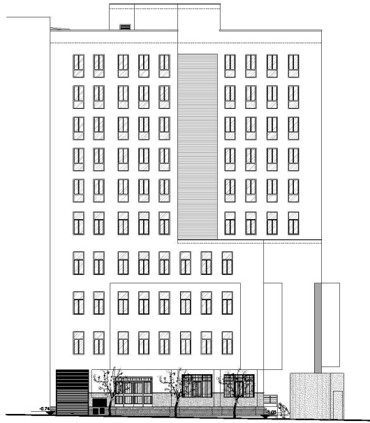
ALZADO PRINCIPAL
