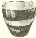
Megaspis transversus , mili, sp. nov.
