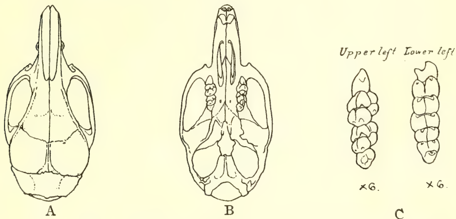
FIG. 2.— Mus (Leggada) ramnadensis : A = skull from above; B = skull from below; x 2; C = Molars.
