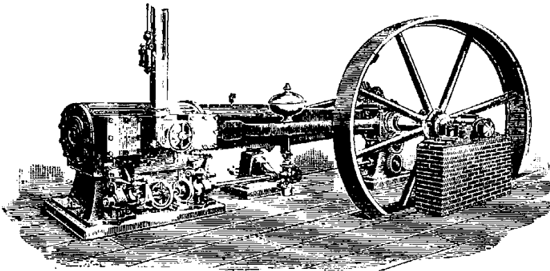
AUTOMATIC CUT-OFF AND SLIDE-VALVE
